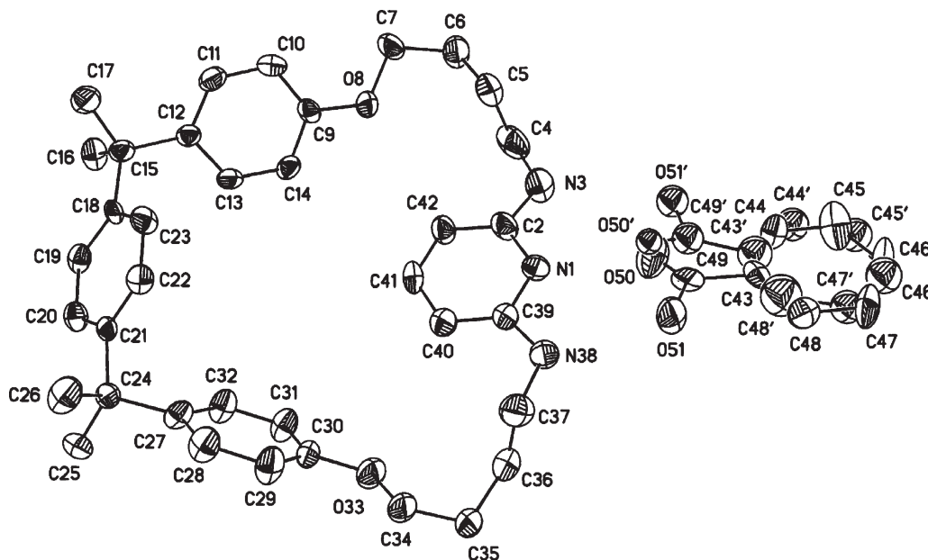
Figure 5. An ORTEP drawing with numbering system for the 1:1 complex of cyclophane 4 and benzoic acid. Thermal ellipsoids are drawn at the 30% probability level. Hydrogen atoms of 4 and benzoic acid are omitted for clarity
