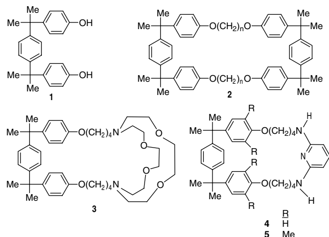
Figure 1. Structures of di- \alpha,\alpha,\alpha',\alpha' -tetramethyl-1,4-benzenedimethanol ( 1 ) and cyclophanes derived therefrom
