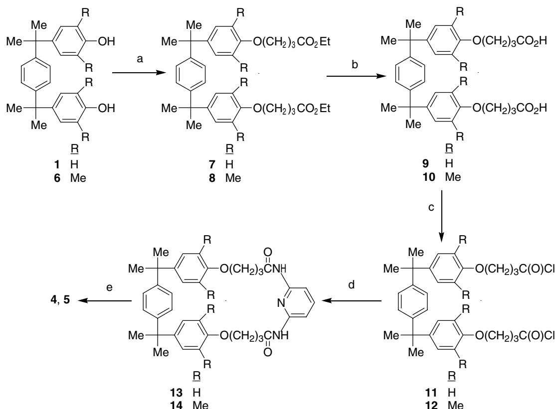
Figure 2. Synthetic scheme for the preparation of ditopic cyclophanes 4 and 5 . Reagents/solvent: (a) ethyl 4-bromobutanoate, K_2CO_3 /acetone; (b) NaOH/aq. EtOH, or H_3O^+ ; (c) SOCl_2 , cat. DMF/benzene; (d) 2,6-diaminopyridine, K_2CO_3 /toluene; (e) BH_3 -THF/THF
