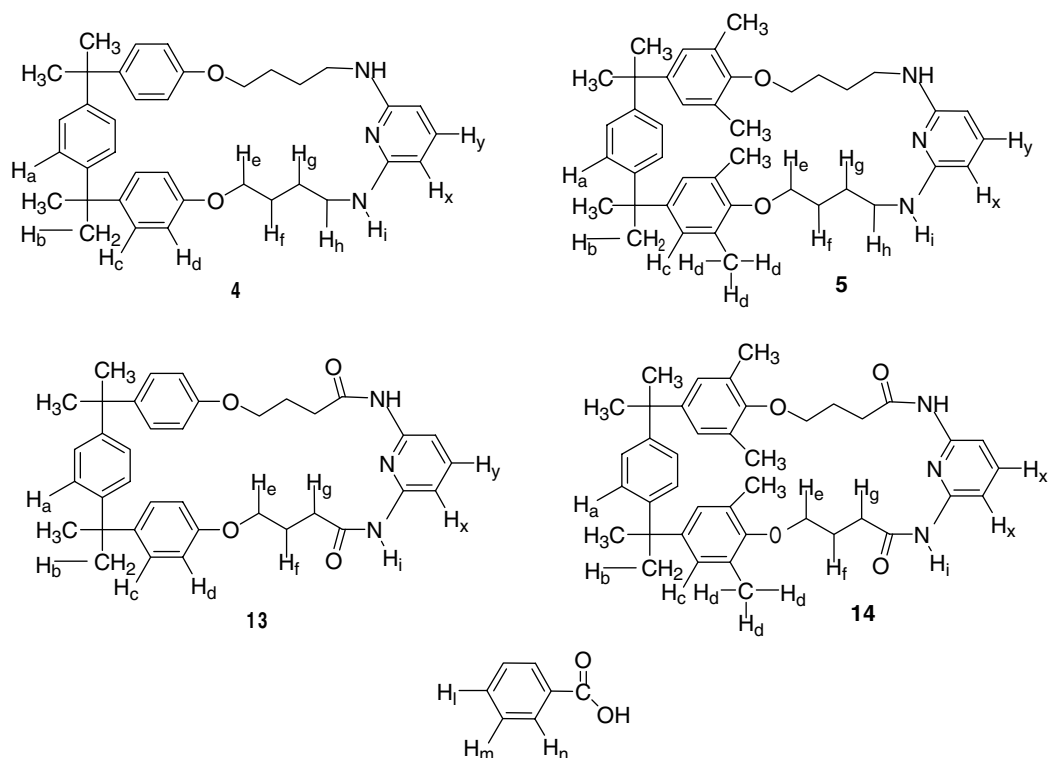
Figure 3. Protons in cyclophane hosts 4 , 5 , 13 and 14 affected by addition of benzoic acid in NMR titration experiments
