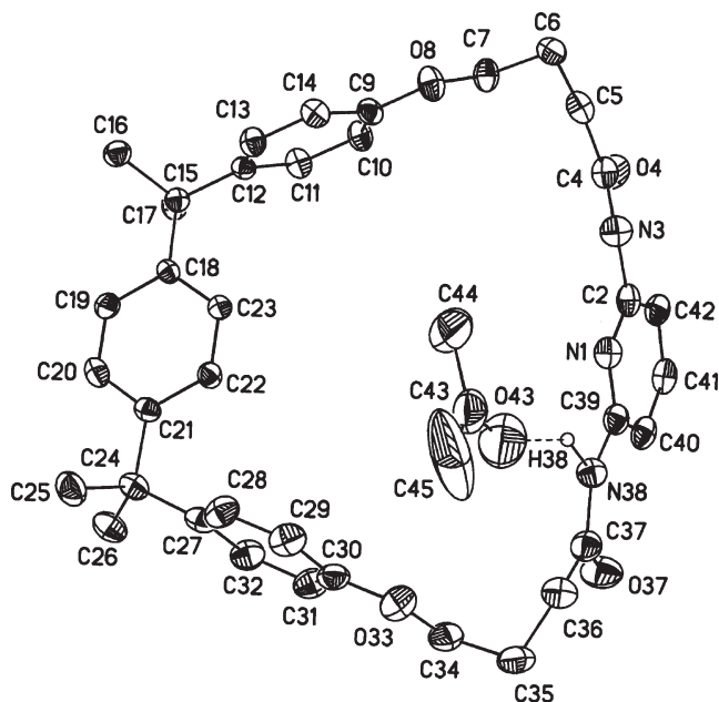
Figure 4. An ORTEP drawing with numbering system for one structure of cyclophane diamide 13 with a solvating molecule of acetone. Thermal ellipsoids are drawn at the 30% probability level. Hydrogen atoms of 13 (except for H38) and the solvating acetone molecule are omitted for clarity
